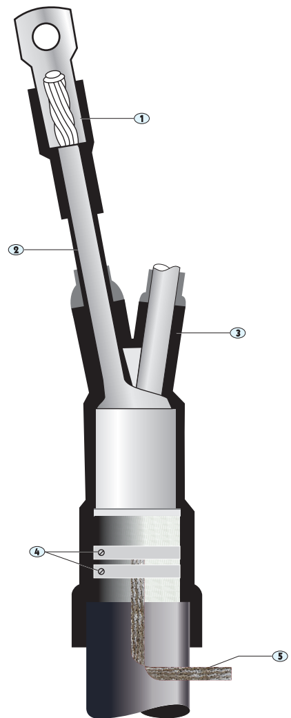
1.1 kV PVC / XLPE Termination
